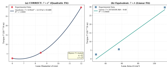
Torque vs Loop Size: Correct Mathematical Relationships
